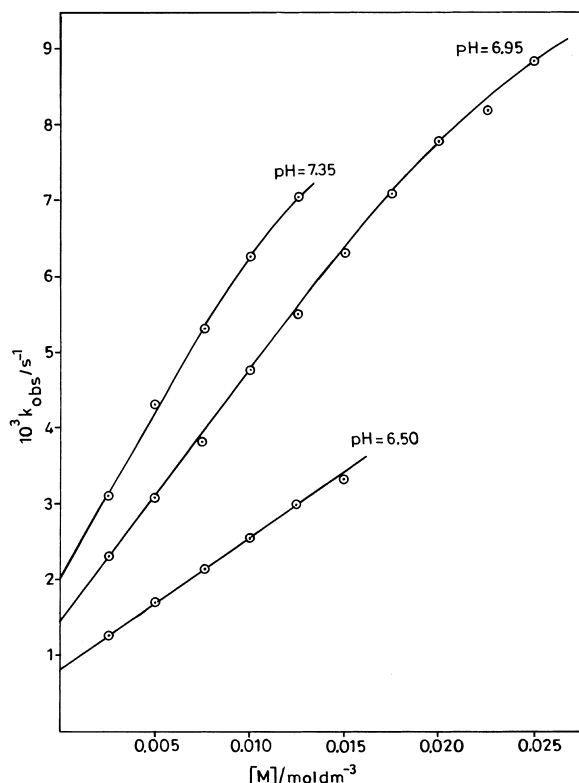
Fig. 2. Variation of Rate Constants ( k_{\text{obs}} ) with Complex Concentration [\text{Co}(\text{OH})(\text{tren})(\text{OH}_2)]^{2+} for PNPG Ester at pH = 6.95, 7.35, 6.50 ( \text{temp} = 35.1 \pm 0.1^\circ \text{C} ).
