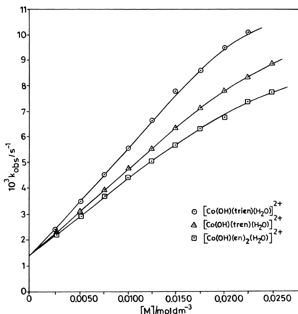
Fig. 1. Variation of Rate Constants ( k_{\text{obs}} ) with Complex Concentration for PNPG Ester at pH = 6.95 \pm 0.05 and \text{temp} = 35.1 \pm 0.1^\circ \text{C} .
